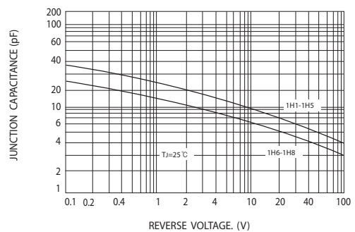
FIG.6-TYPICAL JUNCTION CAPACITANCE
