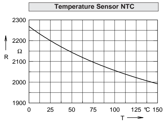
Fig. 11 Typ. thermistorresistance versus temperature
