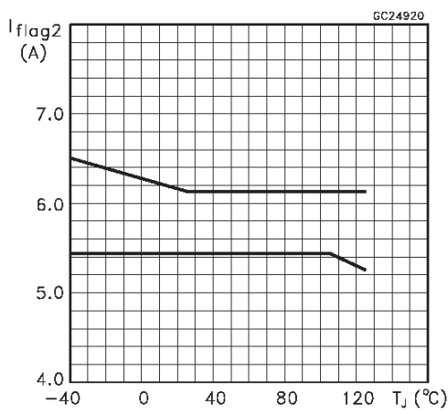
FIGURE 5: I_{flag2} Versus Temperature
