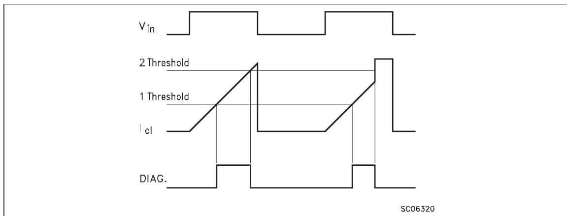
FIGURE 2: Switching Waveforms
