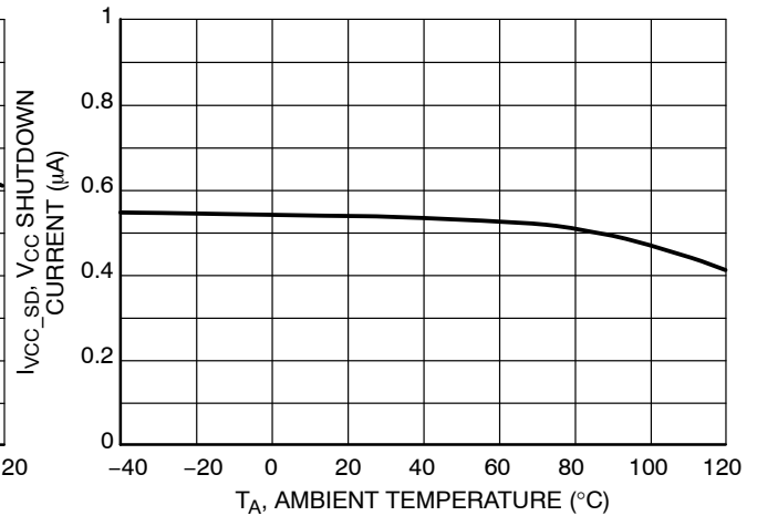
Figure 18. V_{CC} Shutdown Current vs. Ambient Temperature
