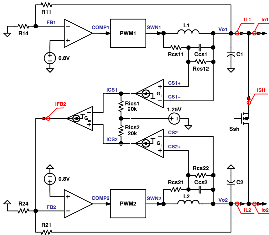
Figure 10. PWM Output Regulation in Two-Phase Mode
