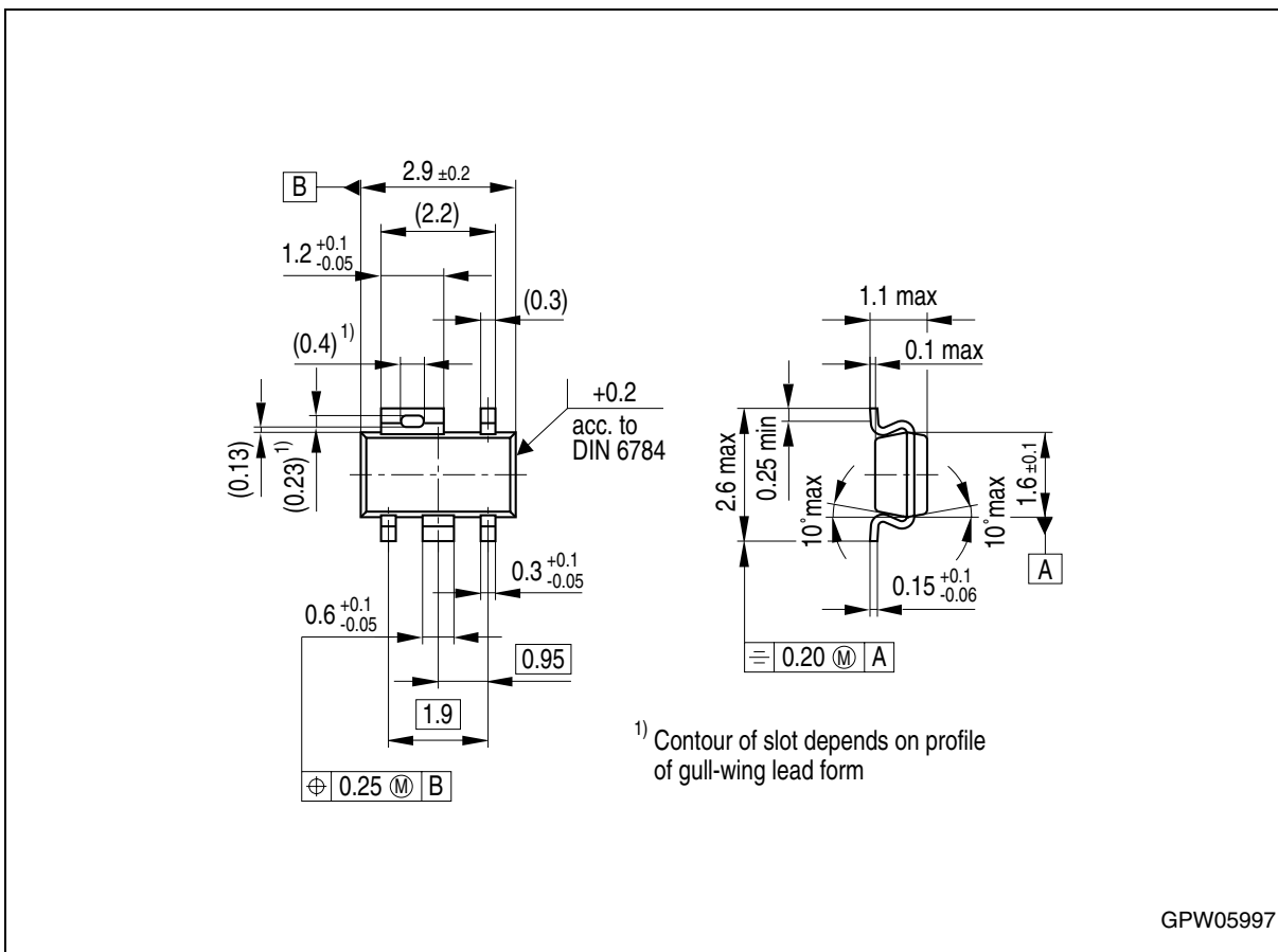
Figure 4 PG-SCT595-5 (Plastic Small Outline)
