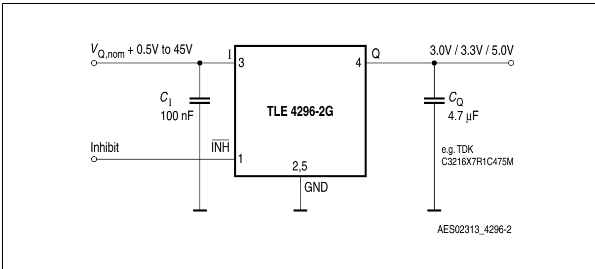
Figure 3 Application Circuit
