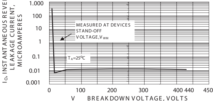
FIG. 7 - TYPICAL REVERSE LEAKAGE CHARACTERISTICS
