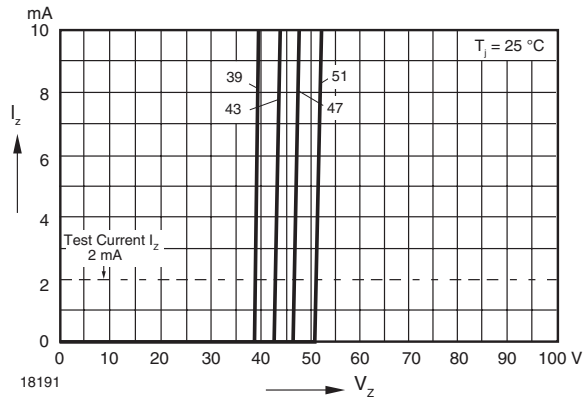
Figure 18. Breakdown Characteristics
