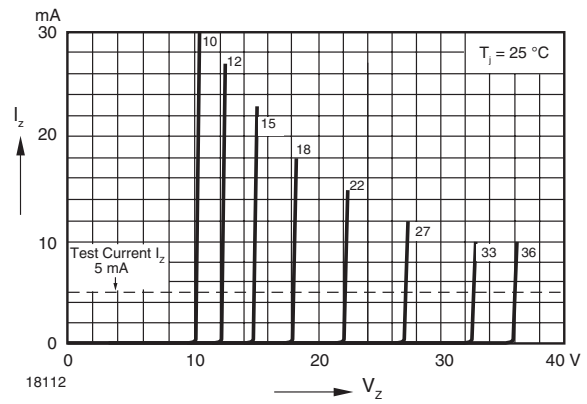
Figure 17. Breakdown Characteristics
