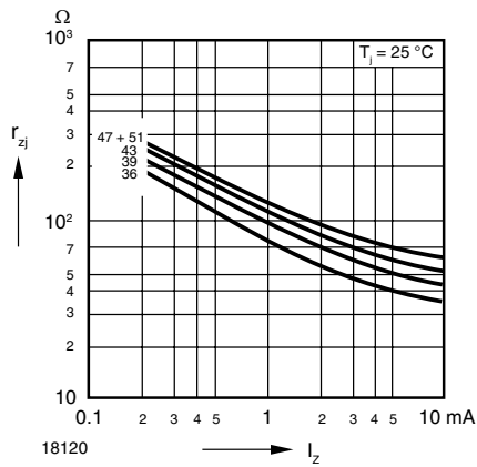
Figure 7. Dynamic Resistance vs. Zener Current
