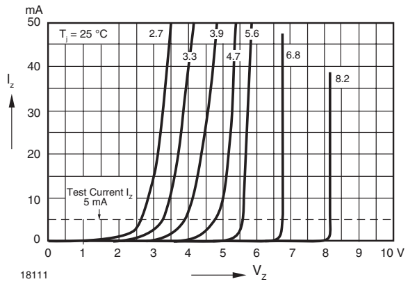
Figure 16. Breakdown Characteristics
