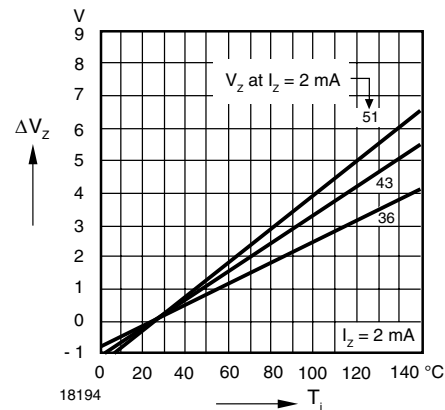
Figure 12. Change of Zener Voltage vs. Junction Temperature
