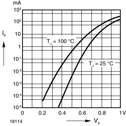
Figure 1. Forward characteristics
