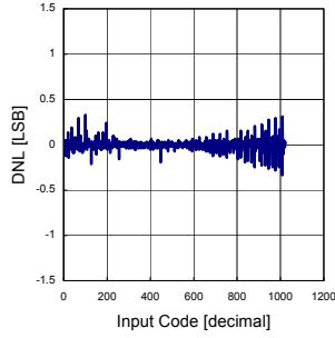
Fig. 5 Differential linearity error (25°C)
