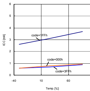
Fig. 10 Circuit current temperature characteristic
