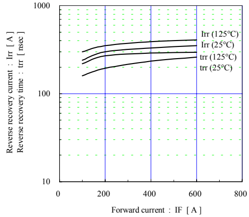
Reverse recovery characteristics (typ.) V cc =600V, V GE =±15V, R g =1.5Ω
