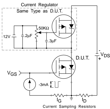
Fig 9b. Gate Charge Test Circuit
