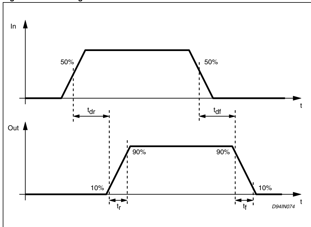
Figure 11. Switching waveforms.
