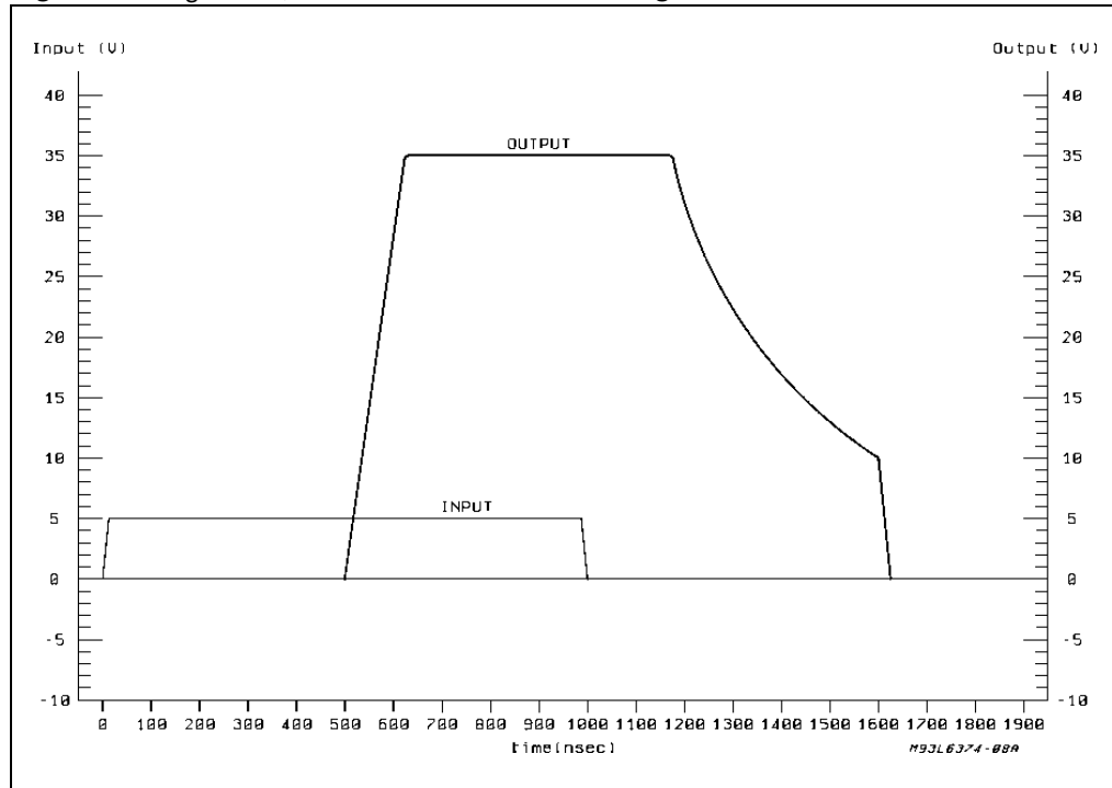
Figure 11. Switching waveforms.
