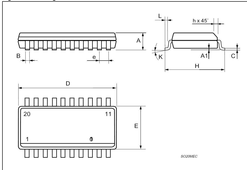
Figure 12. Package dimensions
