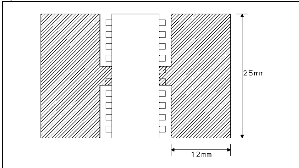
Figure 3. Printed heatsink
