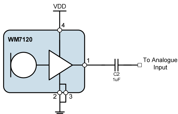
Figure 1 WM7120 Recommended External Components
