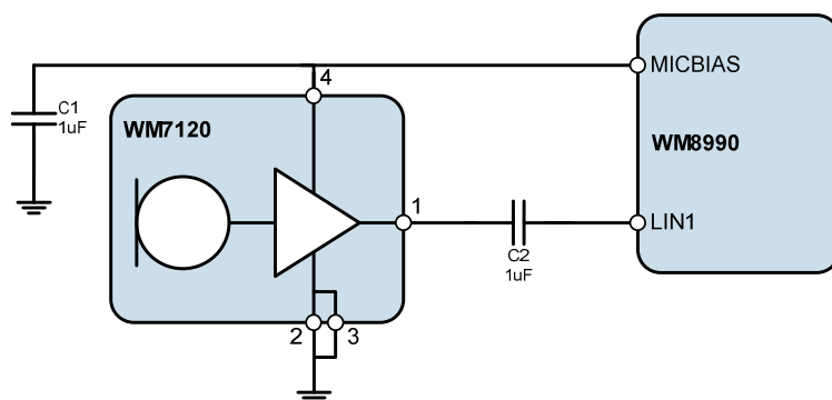
Figure 2 Connection of WM7120 to WM8990
