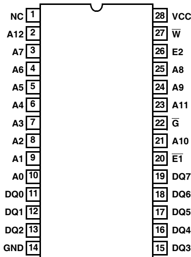
HM-65642/883 (CERDIP) TOP VIEW
