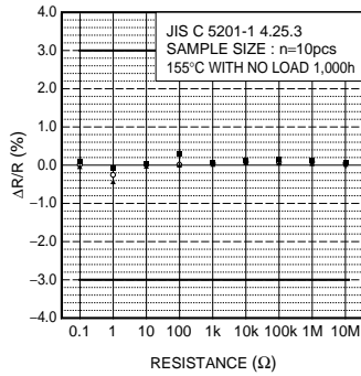
Fig.12 Endurance
