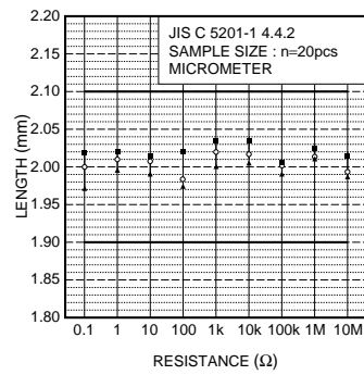
Fig.2 Dimensions (length)
