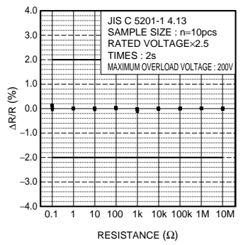
Fig.7 Overload
