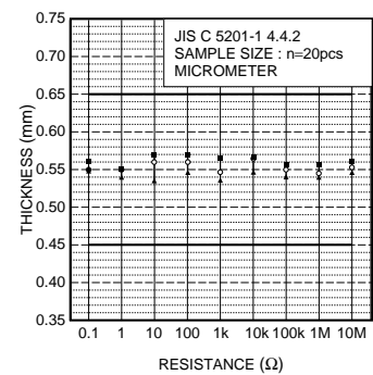
Fig.4 Dimensions (thickness)
