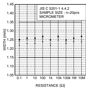
Fig.3 Dimensions (width)
