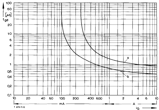
BildFig. 16 Zündverzögerung Gate controlled delay time t_{gd} = f(i_{GM}) , t_{vj} = 25^\circ C , di_G/dt = i_{GM}/1 \text{ ps} a – Maximaler Verlauf/Limiting Characteristic b – Typischer Verlauf/Typical Characteristic
