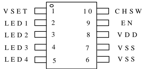
MSOP-10L
