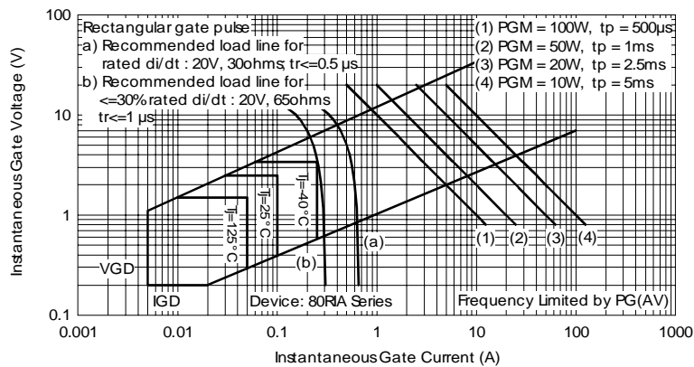
Fig. 9 - Gate Characteristics
