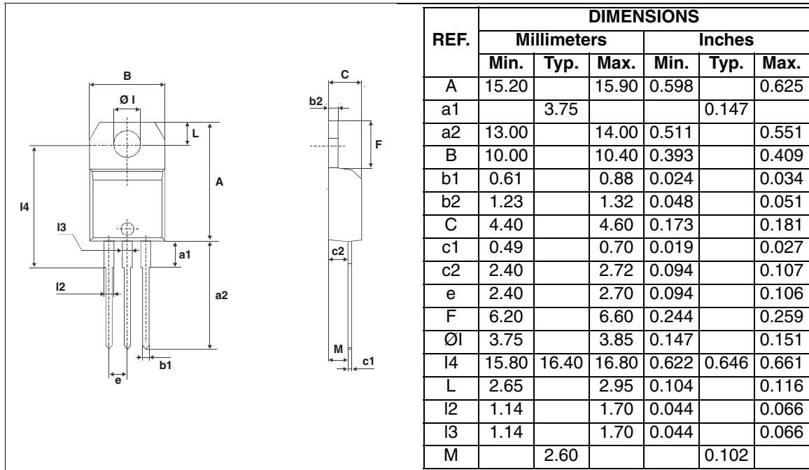
Figure 10: TO-220AB Package Mechanical Data
