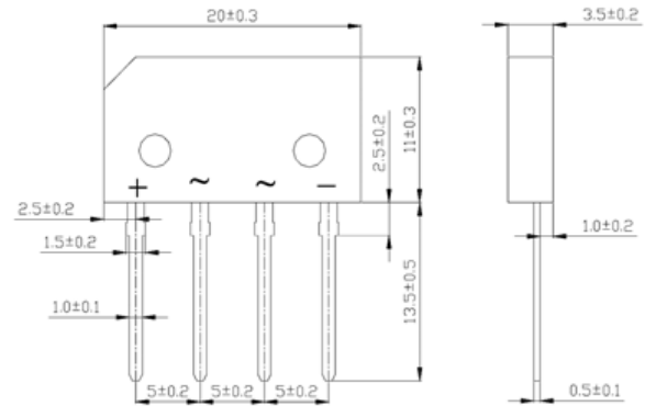
Package outline dimensions in millimeters
