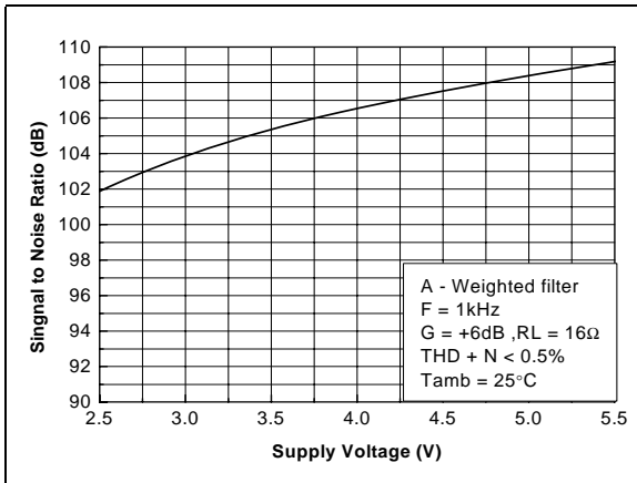
Figure 42. SNR vs. power supply voltage
