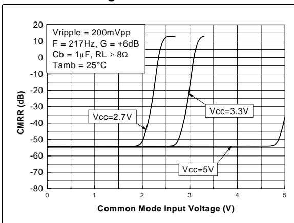
Figure 36. CMRR vs. common mode input voltage
