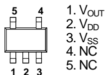
NJU7700/01F
