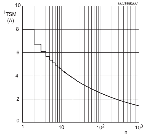
Fig 2. Maximum permissible non-repetitive peak on-state current as a function of number of cycles for sinusoidal currents; typical values.
