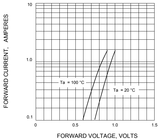
FIG.2 - FORWARD CURRENT AS S FUNCTION OF FORWARD VOLTAGE; TYPICAL VALUES
