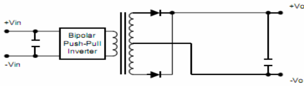
Single Output
