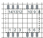
FOOTPRINT DETAILS
