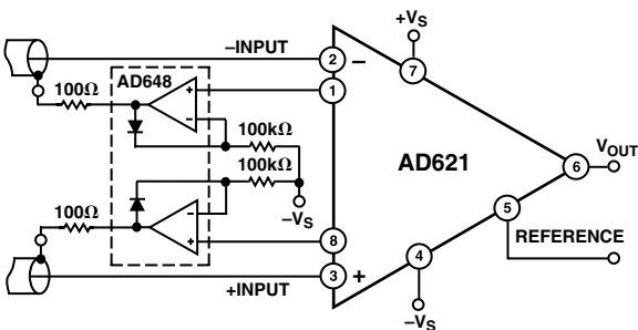
Figure 13. Differential Shield Driver, G = 10
