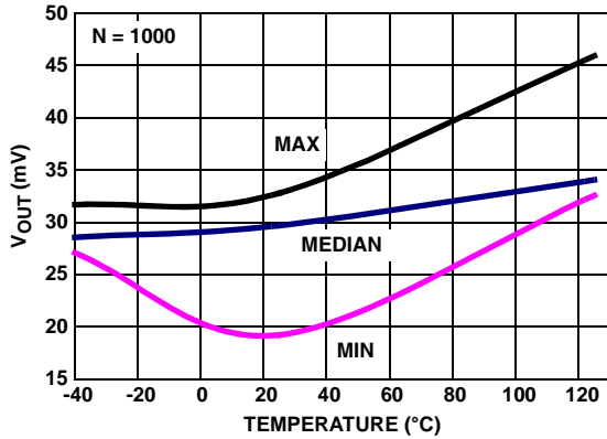
FIGURE 35. ISL28196 V_{OUT} LOW vs TEMPERATURE, V_+ = 5V , V_- = 0V , V_{CM} = 2.5V , R_L = 10k
