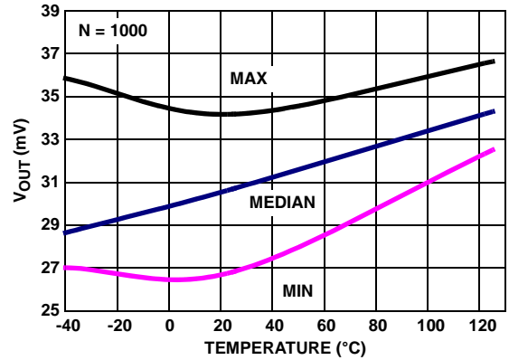
FIGURE 36. ISL28197 V_{OUT} LOW vs TEMPERATURE, V_+ = 5V , V_- = 0V , V_{CM} = 2.5V , R_L = 10k
