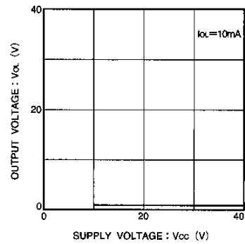
Fig. 3 Output voltage vs. supply voltage characteristic
