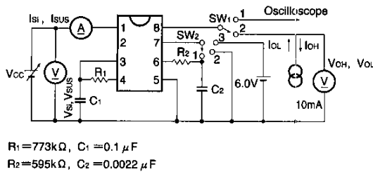
Fig. 5 Measurement circuit (1)
