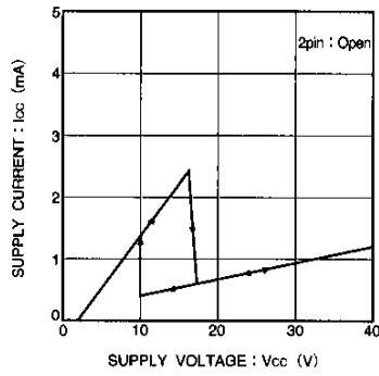
Fig. 1 Supply current vs. supply voltage characteristic
