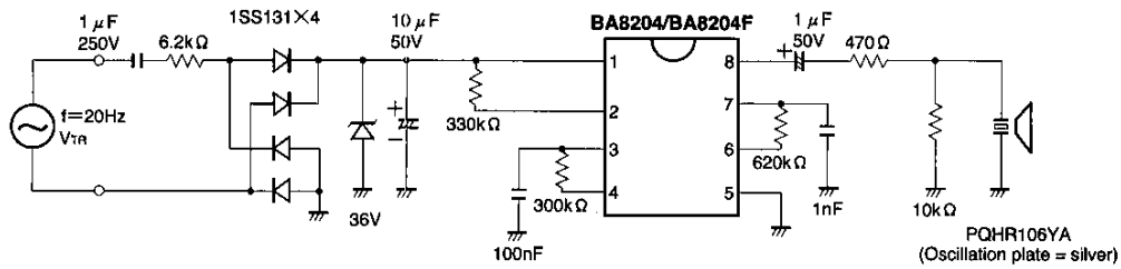
Fig. 4 Ringer threshold voltage measurement circuit
