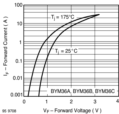
Figure 5. Max. Forward Current vs. Forward Voltage
