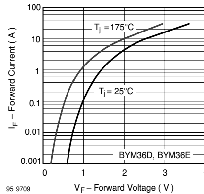
Figure 6. Max. Forward Current vs. Forward Voltage
