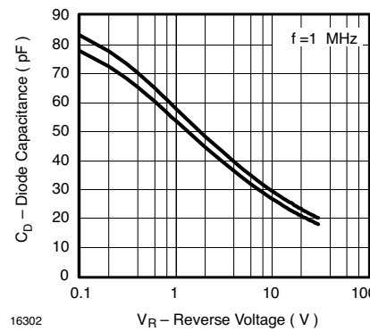
Figure 7. Diode Capacitance vs. Reverse Voltage
