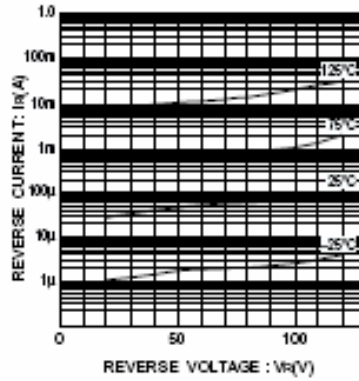
Fig.2 Reverse characteristics
