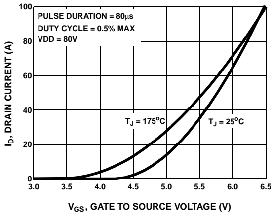
Figure 3. Transfer Characteristics
