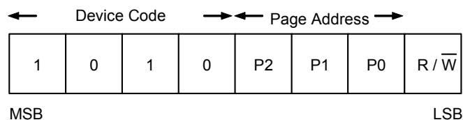
Figure 14 Device Address
