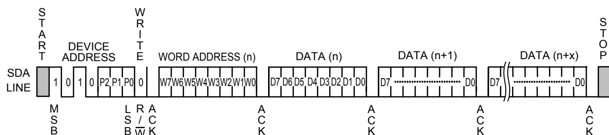
Figure 16 Page Write
