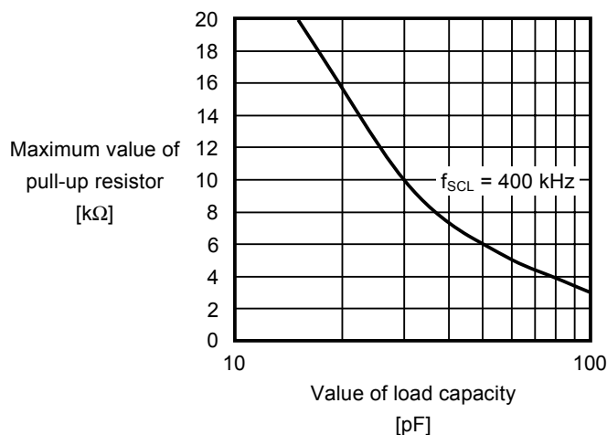
Figure 10 Output Load
