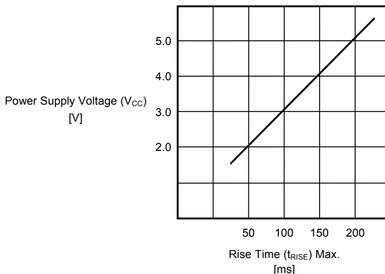
Figure 28 Rise Time of Power Supply Voltage
