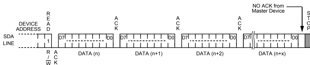
Figure 21 Sequential Read
