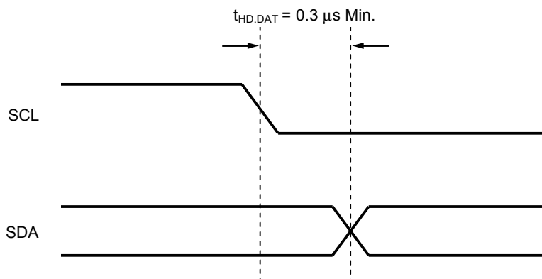
Figure 30 S-24C16C Data Hold Time
