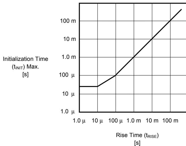
Figure 29 Initialization Time of S-24C16C
