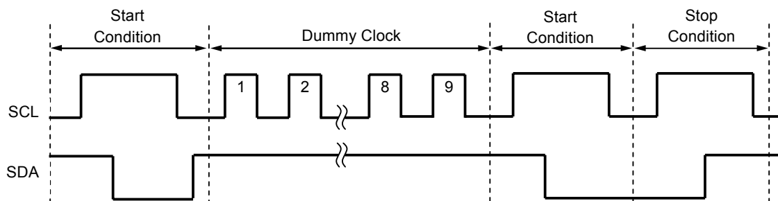
Figure 26 Resetting S-24C16C
