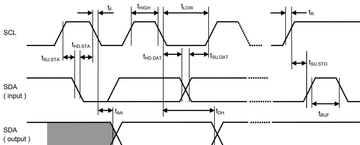
Figure 8 Bus Timing
