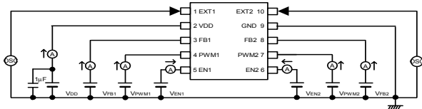
Circuit
