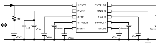
Circuit
