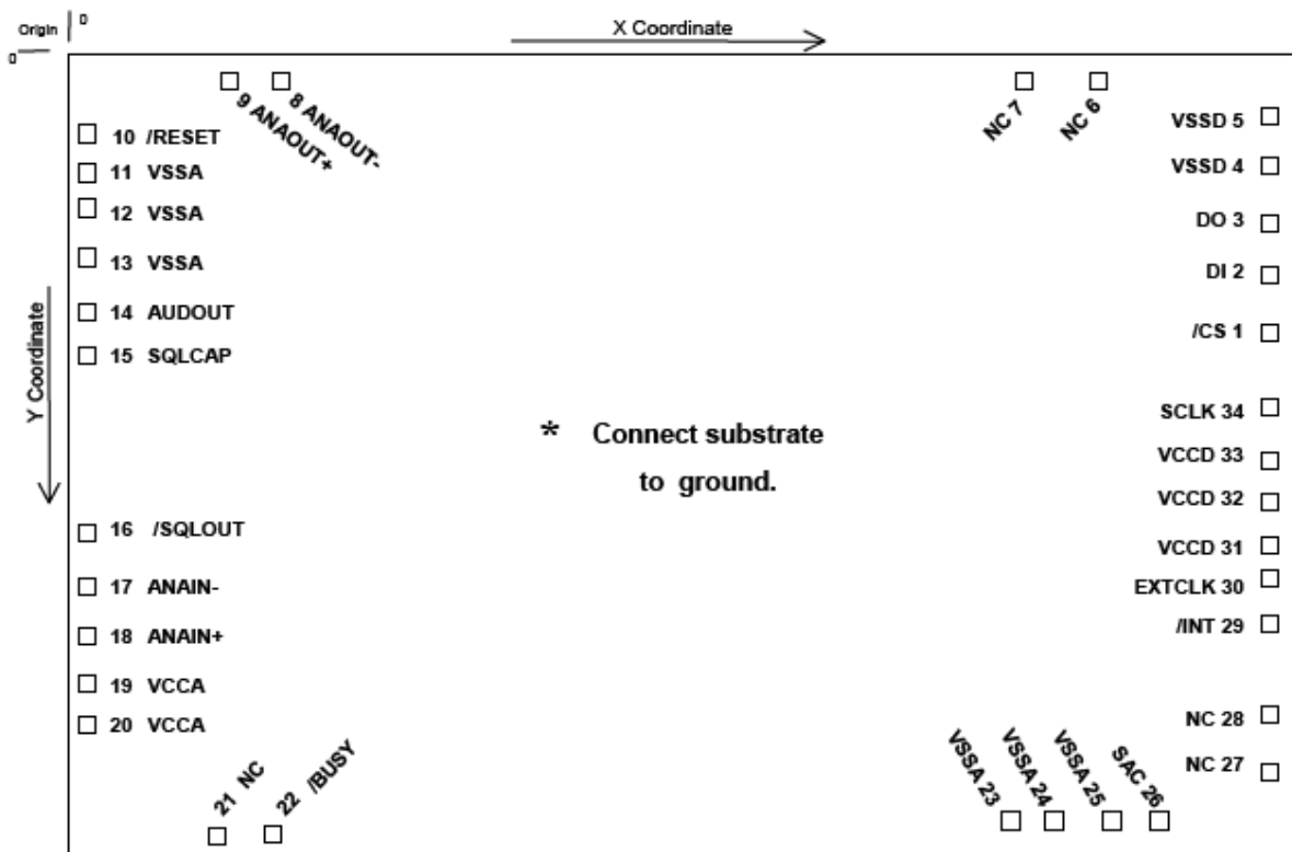
Figure 18 Bond Pad Layout and Coordinates
