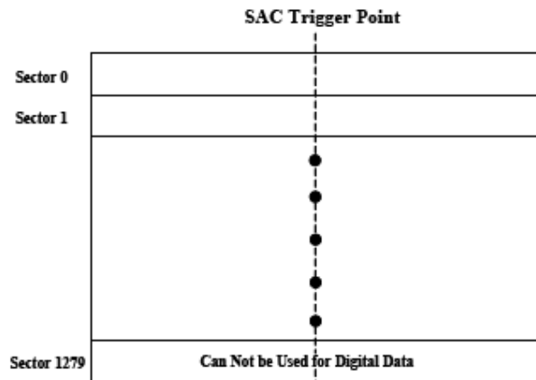
Figure 3 Memory Map.
