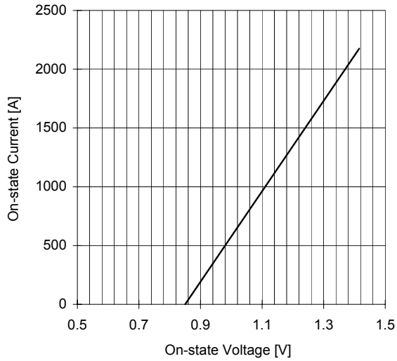
ON-STATE CHARACTERISTIC T j = 150 °C
