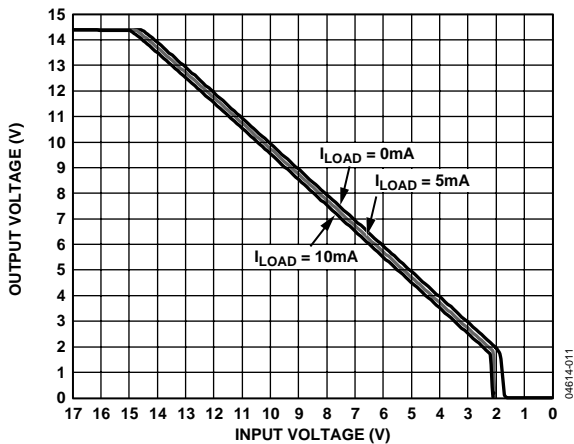
Figure 11. Dropout Characteristics
