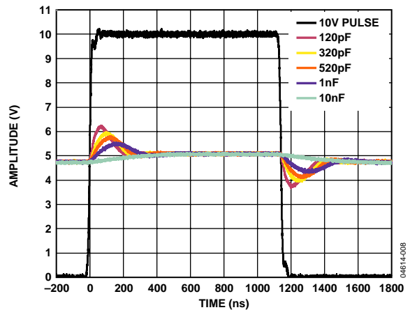
Figure 8. Gamma Buffers Transient Load Response vs. Capacitive Loading
