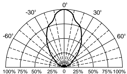
Fig.6 Directive Radiation
