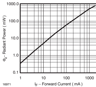
Figure 6. Radiant Power vs. Forward Current
