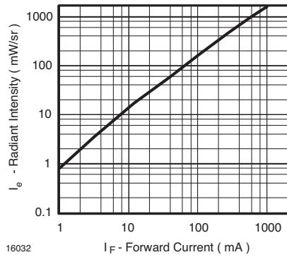
Figure 5. Radiant Intensity vs. Forward Current
