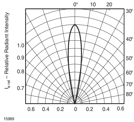
Figure 8. Relative Radiant Intensity vs. Angular Displacement
