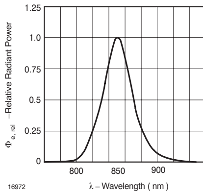
Figure 7. Relative Radiant Power vs. Wavelength
