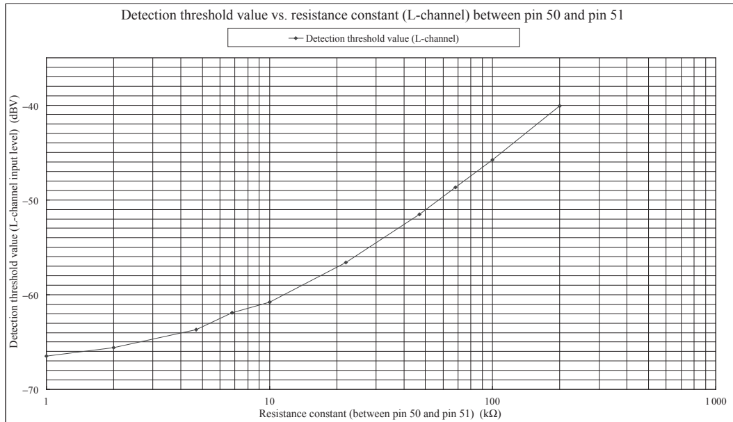
Detection sensitivity threshold values vs. external resistance
