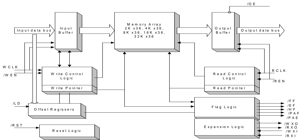
AL4CX36x0 FIFO Block Diagram
