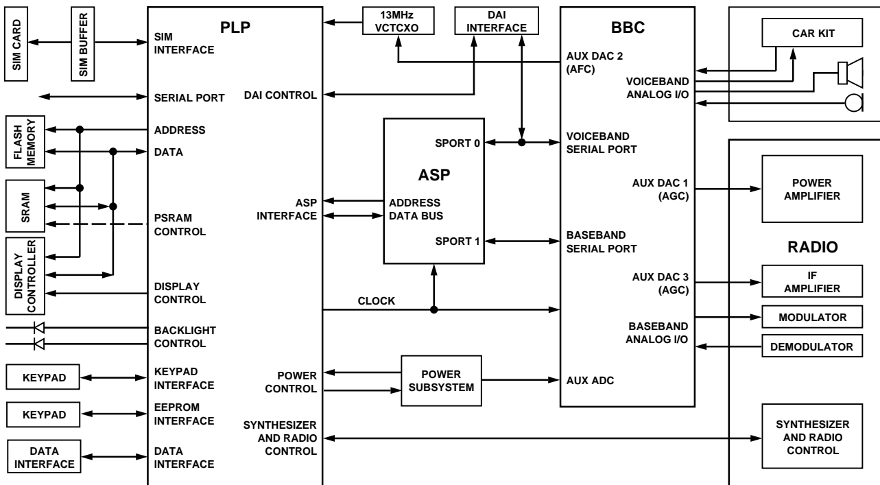
Figure 5. System Interfaces
