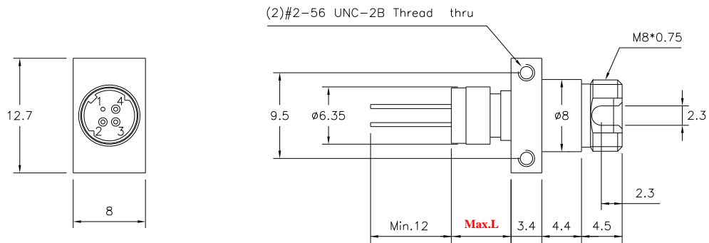
FC RECEPTACLE (BOARD MOUNT) (DL-35XXX-FBX)
