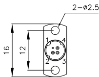
Vertical Flange
