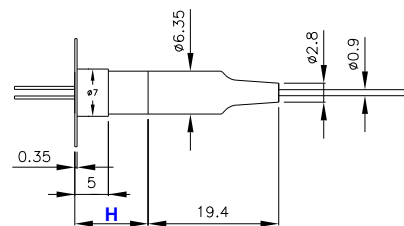
Vertical Flange
