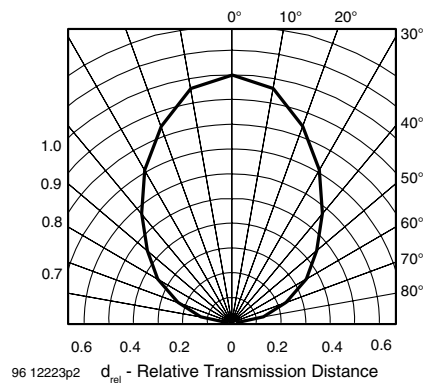
Figure 12. Directivity
