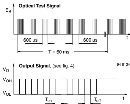
Figure 3. Output Function
