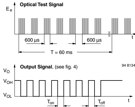
Figure 3. Output Function
