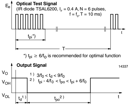
Figure 1. Output Function
