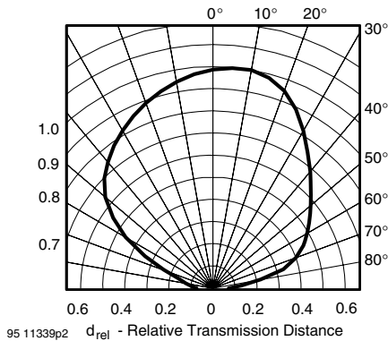
Figure 13. Vertical Directivity \phi_V
