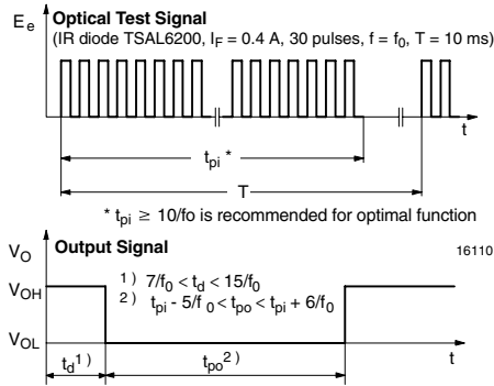
Figure 1. Output Function
