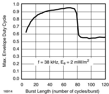
16914 Burst Length (number of cycles/burst) Figure 9. Max. Envelope Duty Cycle vs. Burstlength
