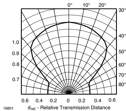
16801 d_{rel} - Relative Transmission Distance Figure 12. Directivity
