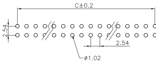
RECOMMEND P.C.B LAYOUT TOP VIEW
