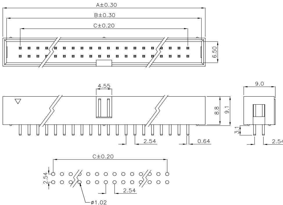
RECOMMEND P.C.B LAYOUT TOP VIEW
