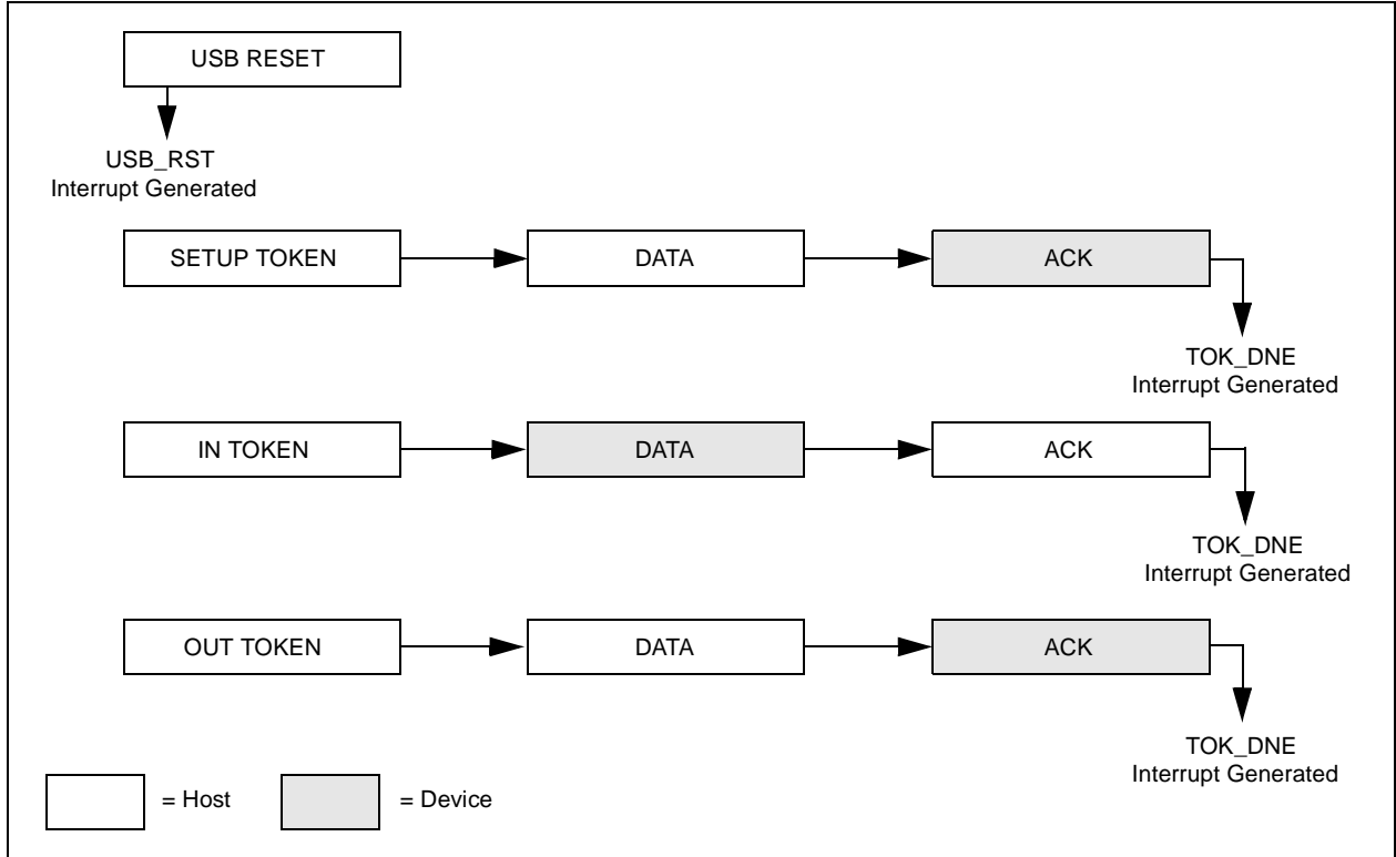
FIGURE 10-1: USB TOKENS
