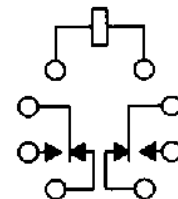
TERMINAL VIEW
